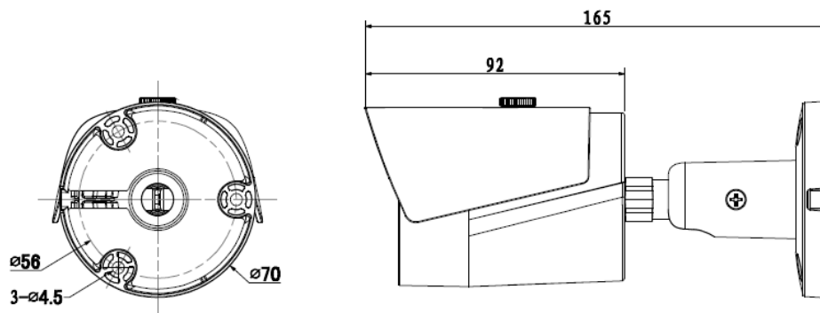
Figure 2-3 Model C (mm)
