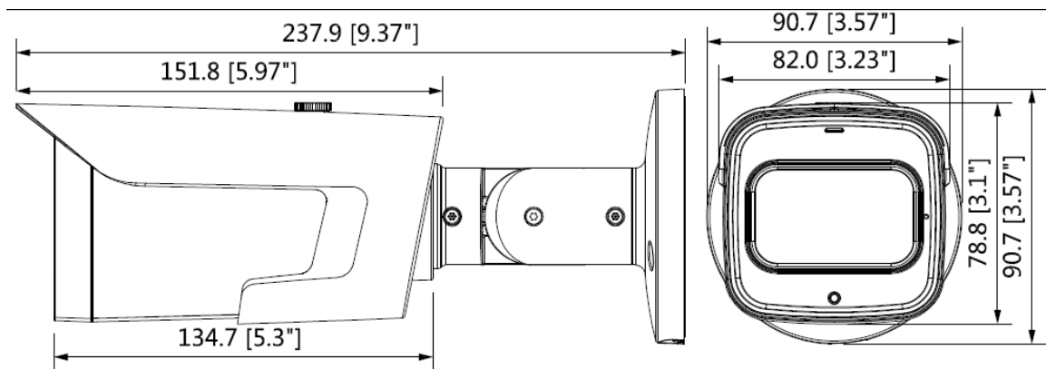
Figure 2-4 Model D (mm [in]) and Model E (mm [in])
